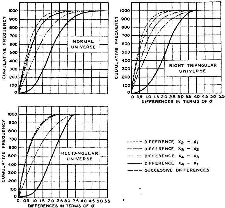
FIG. 72.—HOW DISTRIBUTIONS OF ORDERED DIFFERENCES DEPEND UPON THE UNIVERSE.
