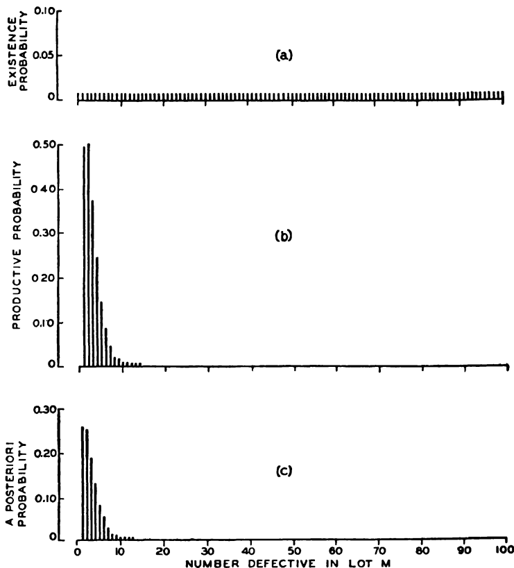
FIG. 122.—RELATION BETWEEN PROBABILITIES.
