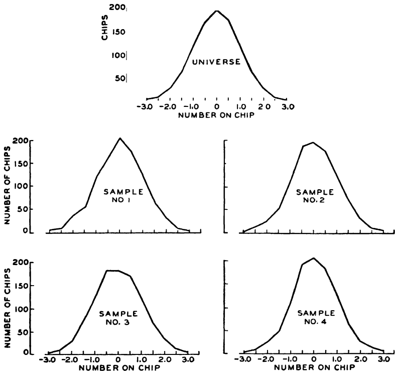
FIG. 56.—SAMPLING FLUCTUATIONS UNDER CONTROLLED CONDITIONS.
