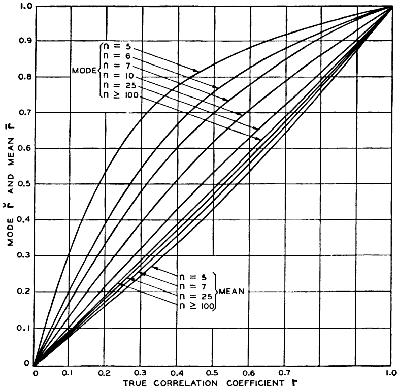
FIG. 78.—RELATIONSHIP OF MODAL VALUE \check{r} AND EXPECTED VALUE \bar{r} IN SAMPLES OF SIZE n FROM A NORMAL UNIVERSE WITH CORRELATION COEFFICIENT \tau .
