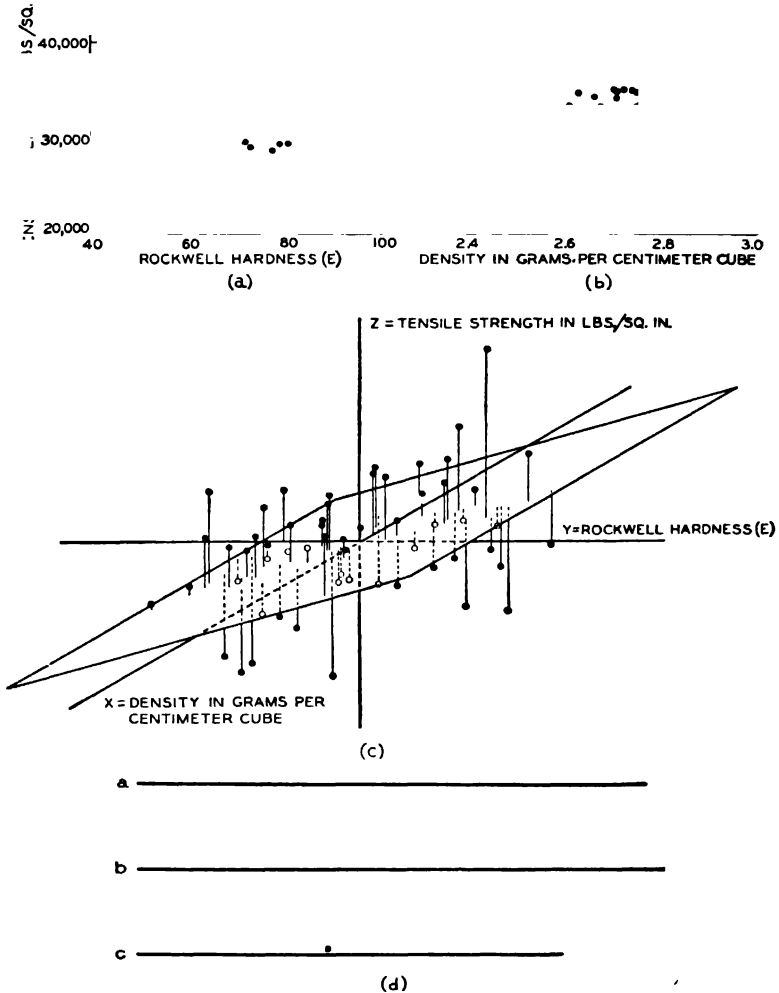
FIG. 14.—HOW CONTROL MAKES POSSIBLE IMPROVED QUALITY THROUGH REDUCTION IN TOLERANCE LIMITS.
