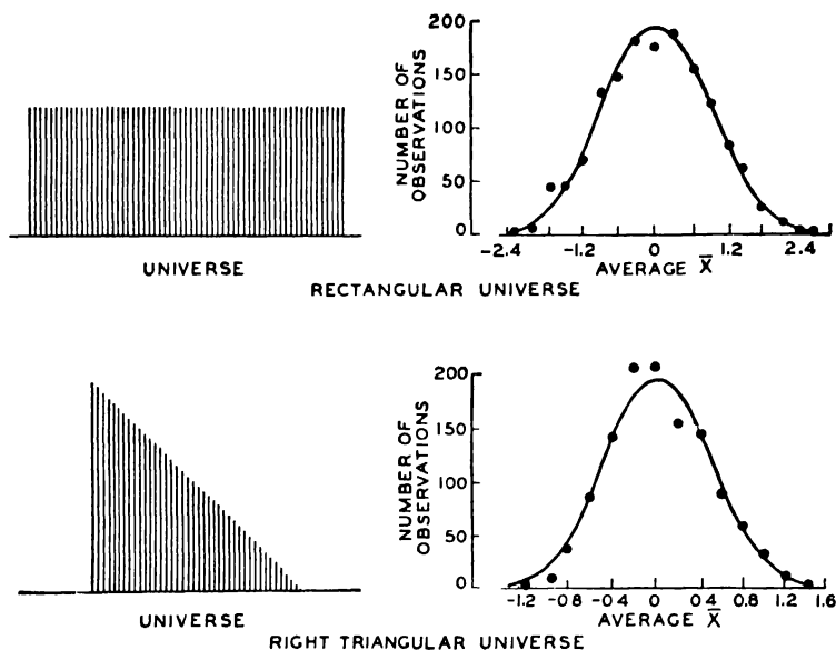
FIG. 59.—UNIVERSES AND DISTRIBUTIONS OF AVERAGES FROM RECTANGULAR AND RIGHT TRIANGULAR UNIVERSSES.
