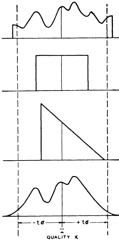
FIG. 92.—FOUR UNIVERSES OF EFFECTS SATISFYING THE SPECIFICATION THAT THE EXPECTED VALUE SHALL BE \bar{X} AND STANDARD DEVIATION SHALL BE \sigma .
