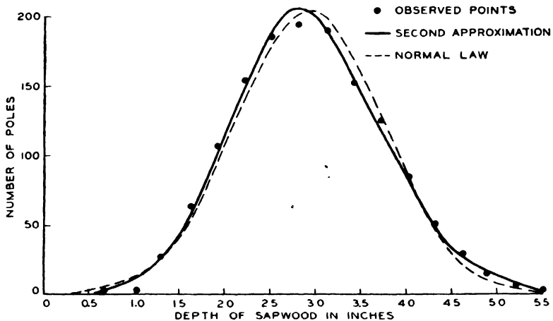
FIG. 32.—SIGNIFICANCE OF AVERAGE, STANDARD DEVIATION, AND SKEWNESS.
