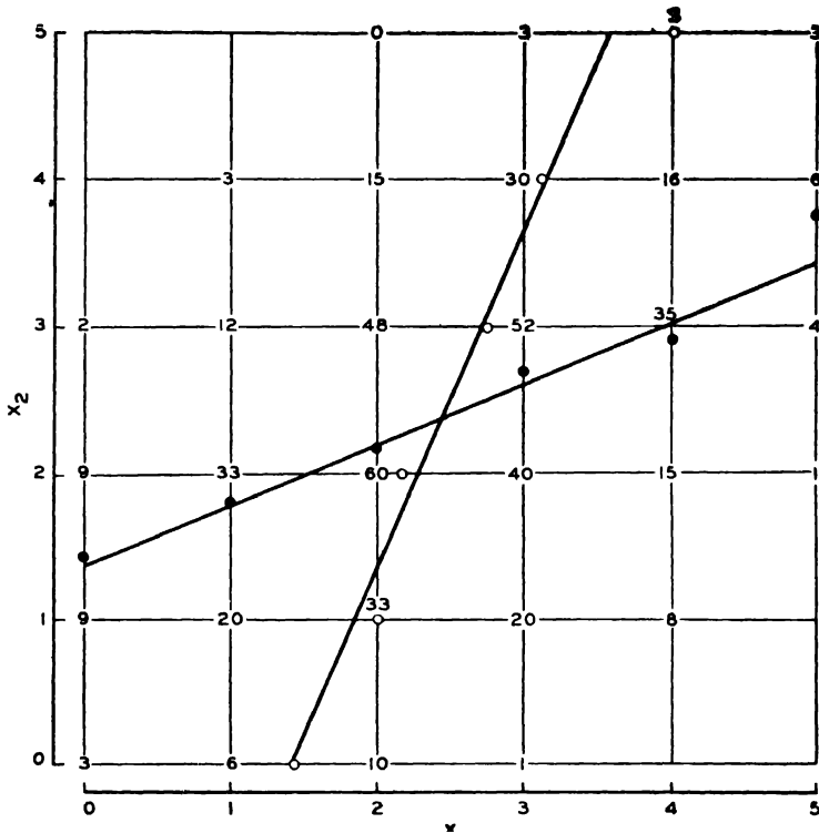
FIG. 81.—SCATTER DIAGRAM AND LINES OF REGRESSION FOR 500 OBSERVED VALUES.
