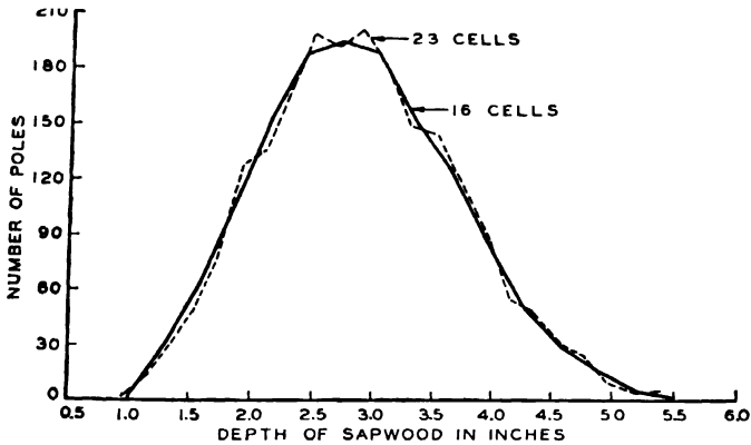
FIG. 28.—EFFECT OF CLASSIFICATION ON GRAPHICAL REPRESENTATION.
