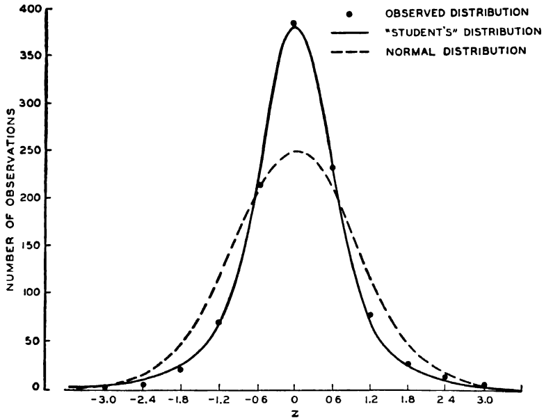
FIG. 62.—COMPARISON OF "STUDENT'S" DISTRIBUTION WITH THE NORMAL LAW AND WITH THE OBSERVED VALUES OF z FOR SAMPLES OF FOUR.
