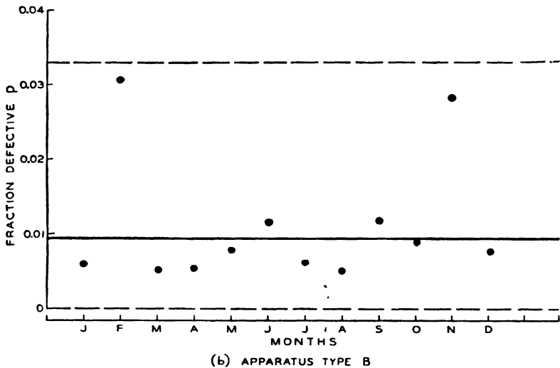
FIG. 4.—SHOULD THESE VARIATIONS BE LEFT TO CHANCE? a —"No." b —"Yes."
