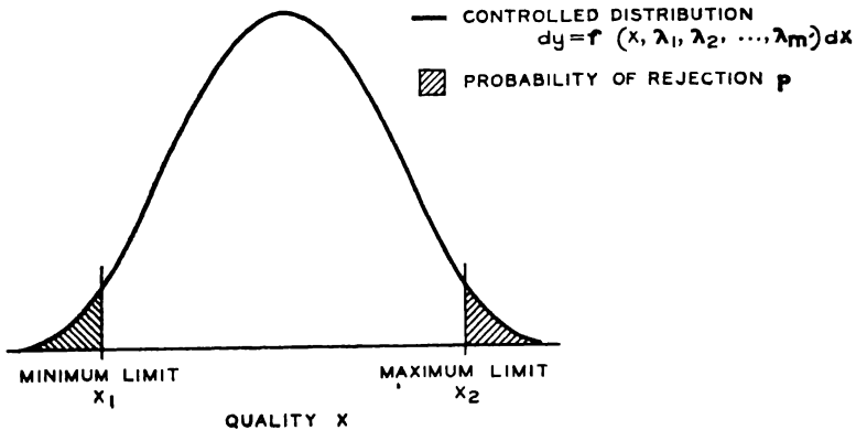
FIG. 85.—TOLERANCE ON FRACTION DEFECTIVE FOR CONTROLLED QUALITY.
