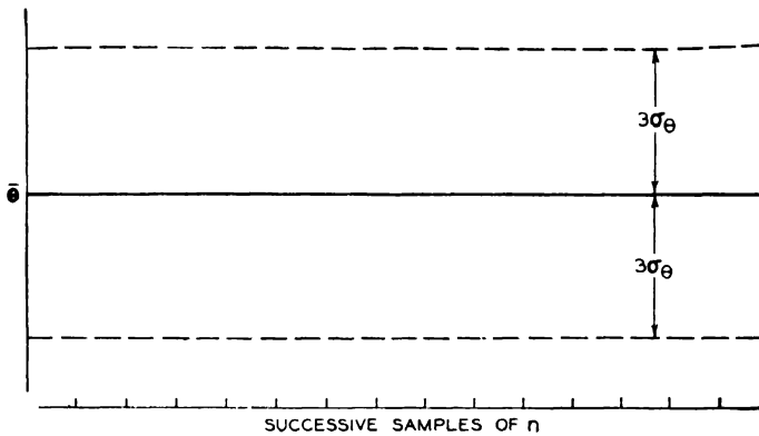
FIG. 100. SIMPLE FORM OF CONTROL CHART.
