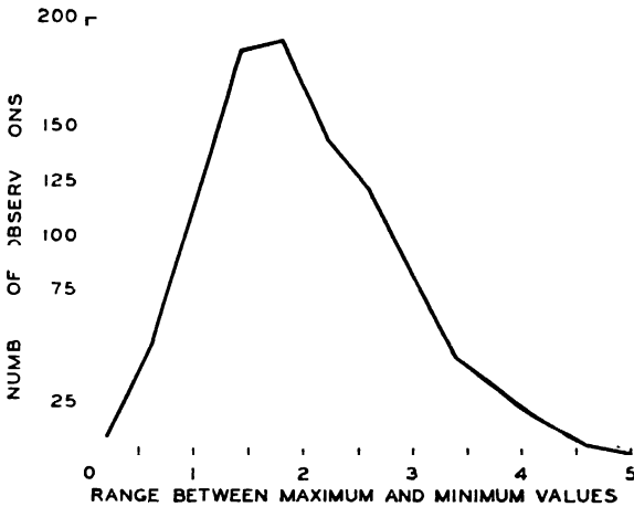
FIG. 69.—OBSERVED DISTRIBUTION OF 1,000 RANGES IN SAMPLES OF FOUR DRAWN FROM A NORMAL UNIVERSE.
