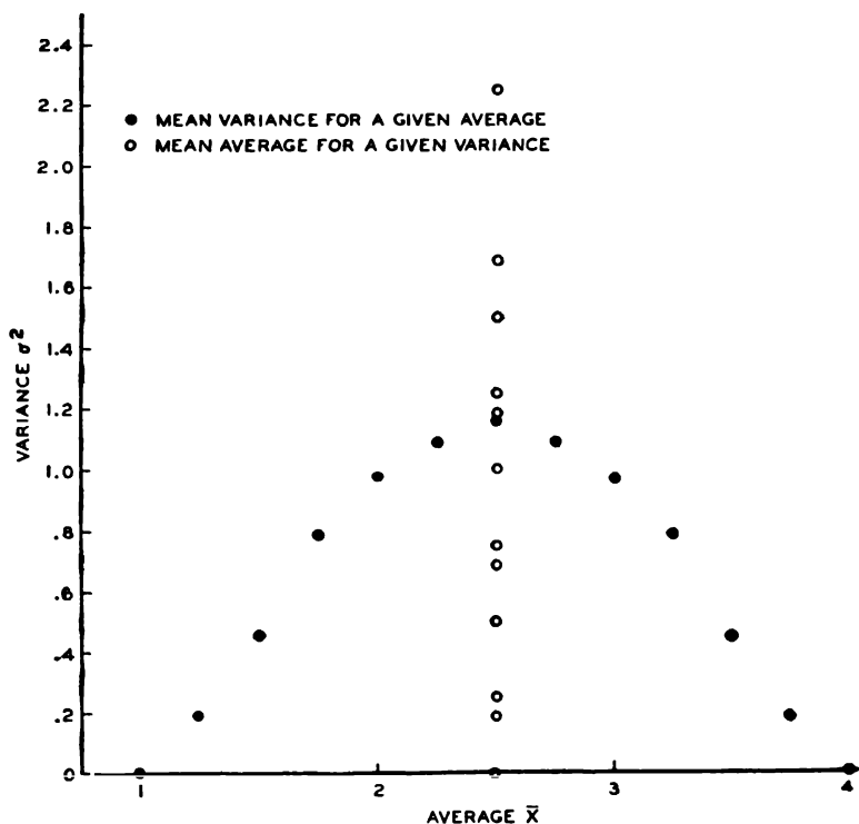
FIG. 66.—SCATTER DIAGRAM FOR AVERAGES AND VARIANCES OF ALL POSSIBLE SAMPLES OF FOUR FROM UNIVERSE 1, 2, 3, 4.
