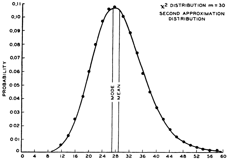
FIG. 74.—DISTRIBUTION OF \chi^2 FOR m = 30 .
