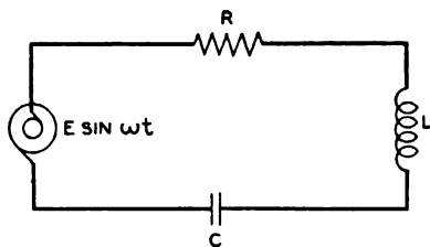
FIG. 41.—EXAMPLE OF CONTROLLED PHENOMENON OBEYING AN EXACT LAW.
