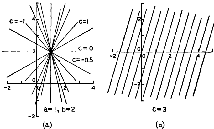
FIG. 34.—GRAPH OF FUNCTION Y = c(X - a) + b SHOWING SIGNIFICANCE OF PARAMETERS a , b , AND c .
