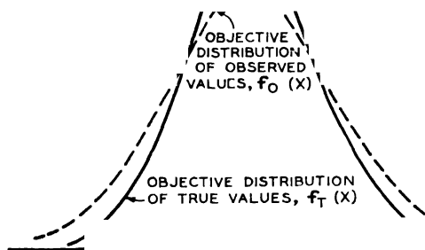
FIG. 134.—EFFECT OF ERROR OF MEASUREMENT.
