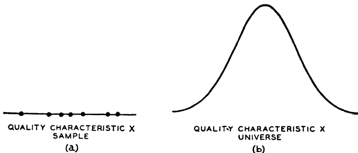
FIG. 23.—SCHEMATIC RELATION BETWEEN SAMPLE AND UNIVERSE.
