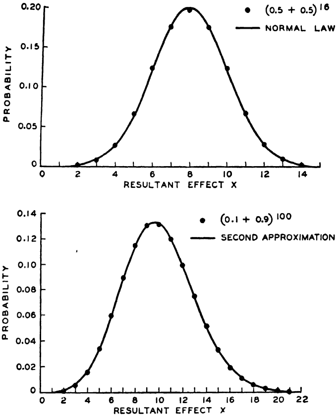
FIG. 54.—APPROACH TO NORMALITY WITH INCREASE IN NUMBER OF CAUSES.
