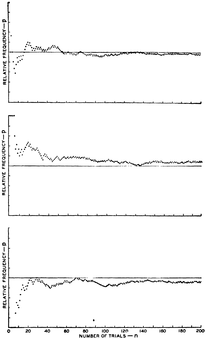
FIG. 128.—BASIC INFORMATION FOR STATISTICAL PREDICTION.
