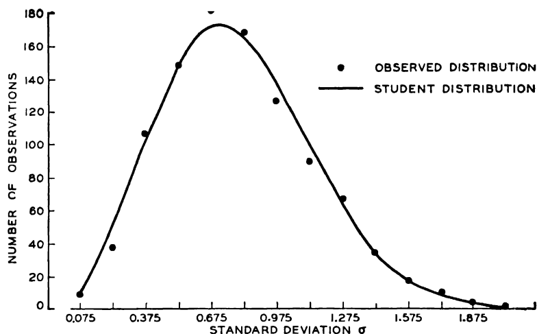
FIG. 60.—DISTRIBUTION OF STANDARD DEVIATIONS IN SAMPLES OF FOUR DRAWN FROM NORMAL UNIVERSE
