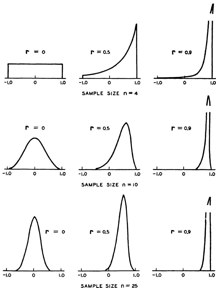
FIG. 76.—TYPICAL DISTRIBUTIONS OF CORRELATION COEFFICIENT.
