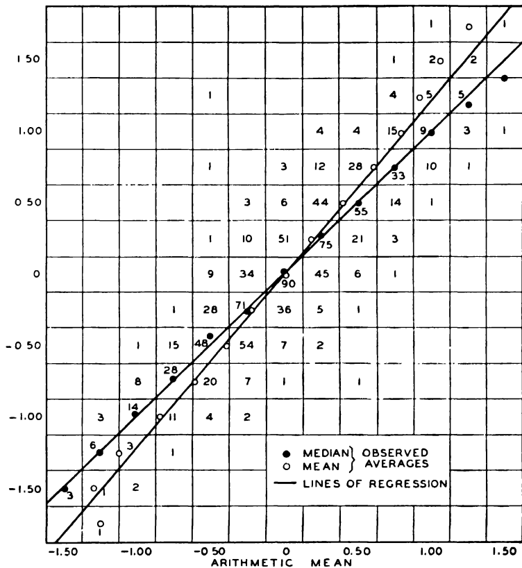
FIG. 95.—SCATTER DIAGRAM OF CORRELATION BETWEEN MEDIANS AND MEANS.
