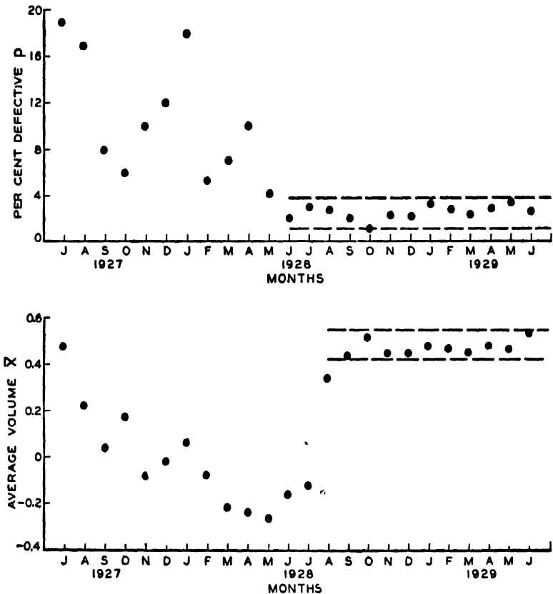
FIG. 11.—APPROACH TO STABLE EQUILIBRIUM OR CONTROL AS ASSIGNABLE CAUSES ARE WEEDED OUT, THUS REDUCING THE NEED FOR INSPECTION.
